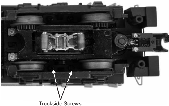
Figure 9: Truckside Screws
