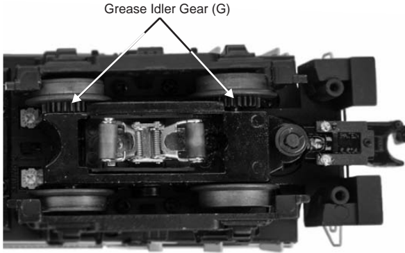
Figure 8: Greasing the Idler Gears
